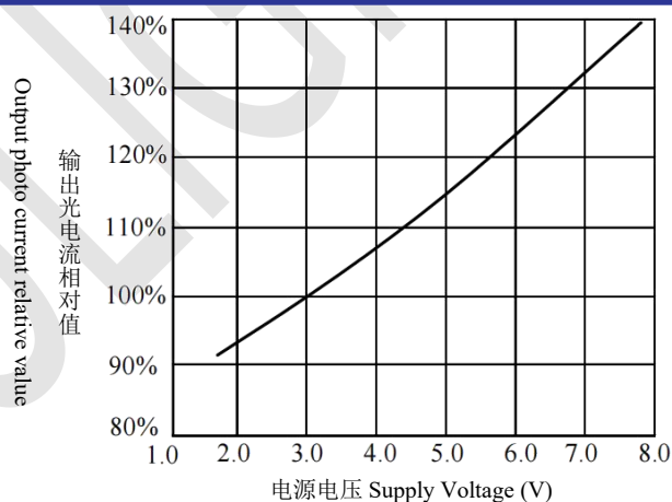
Relative output photo current vs. Supply Voltage
