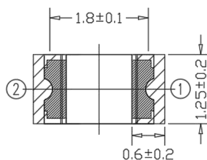
Recommend Soldering Pad
