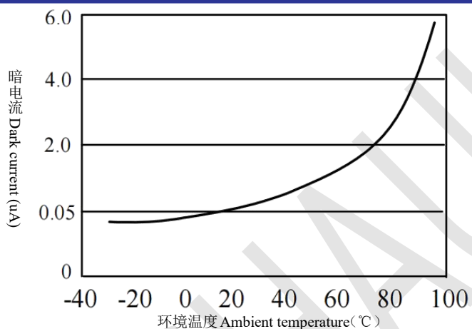
Dark current vs. Ambient Temperature
