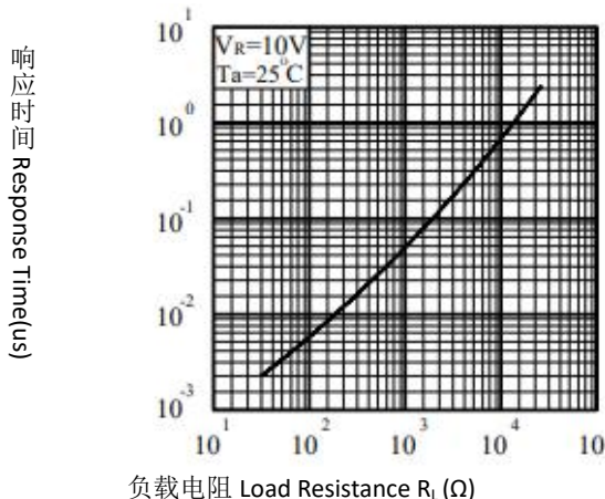
Response Time vs. Load Resistance
