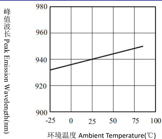
Peak Emission Wavelength vs. Ambient Temperature
