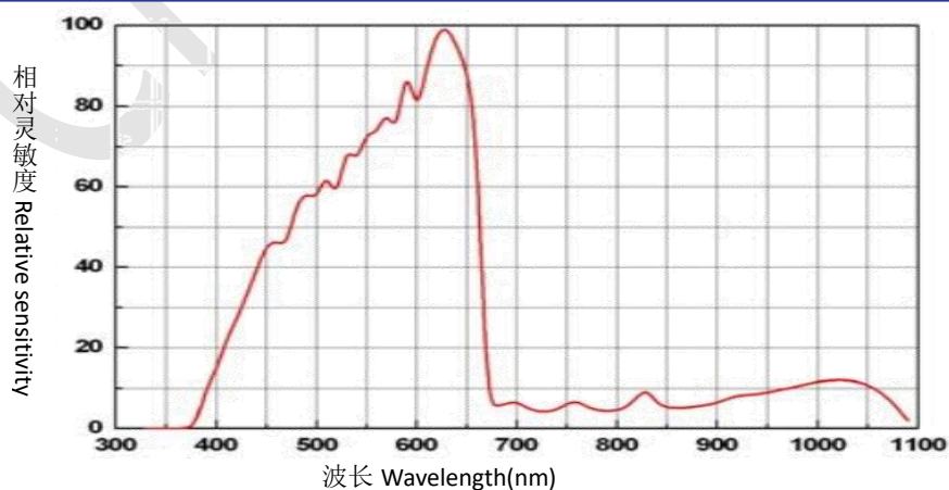
Spectral Response Curve
