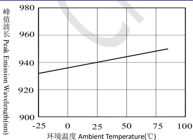
峰值波长与环境温度的关系 Peak Emission Wavelength vs. Ambient Temperature
