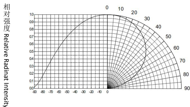
Relative Radiant Intensity vs. Angular Displacement
